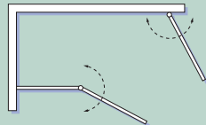
DFY10 half height fixed panel & post & bi-part doors across corner
