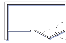
DFY5 half height fixed panel & post & bi-fold door either hand
