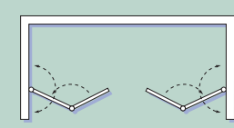
DFY15 half height twin bi- fold doors across front
